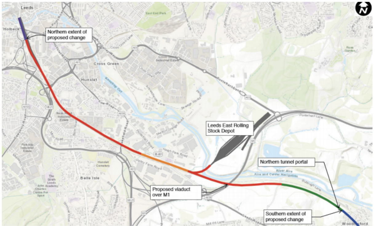
Figure 1 – Revised HS2 route to Leeds
